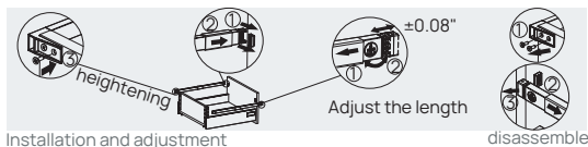
Heightening rod installation, adjustment and removal
