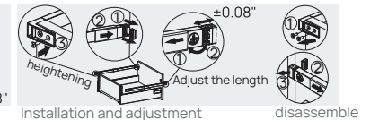
Heightening rod installation, adjustment and removal
