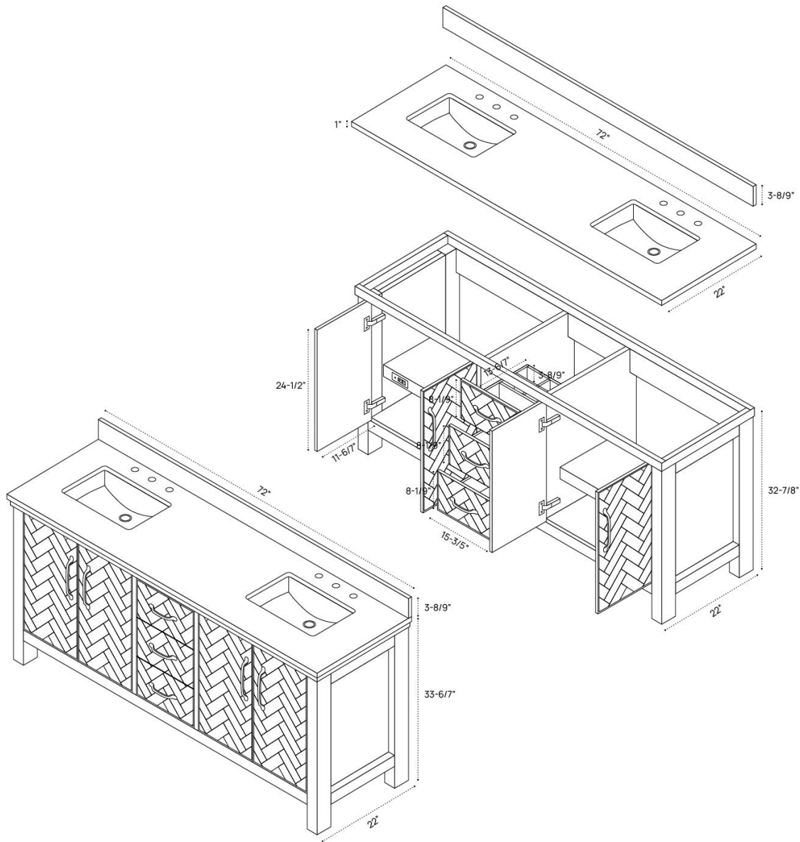
3D VIEW
