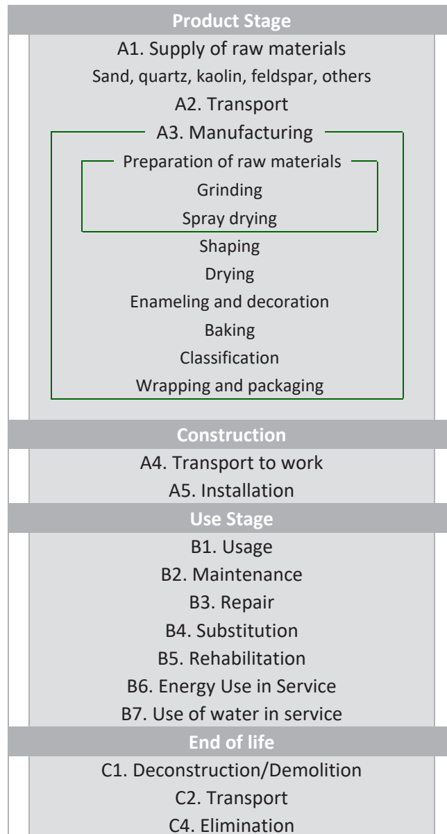
Figure 1. Diagram with system boundaries, steps and processes for the production of 1 m 2 of BIa (8 mm to 12 mm) ceramic tile
